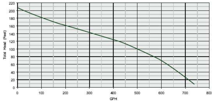
PERFORMANCE CURVE
